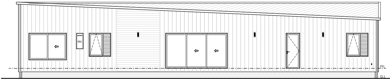
ELEVATE TILT 150 SHOWHOME - ELEVATIONS
