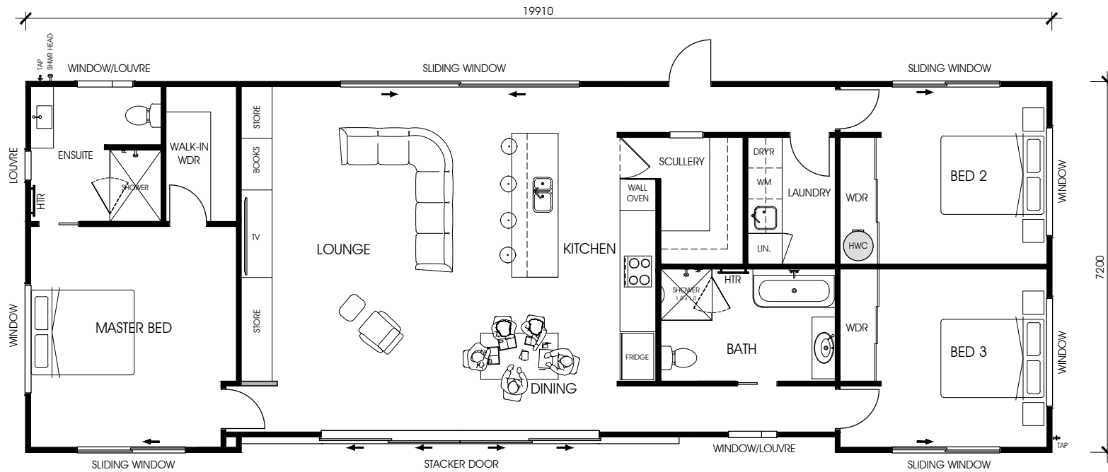
BOX 140 | BARN 140 - DETAILED FLOOR PLAN LIVING AREA: 140m 2
