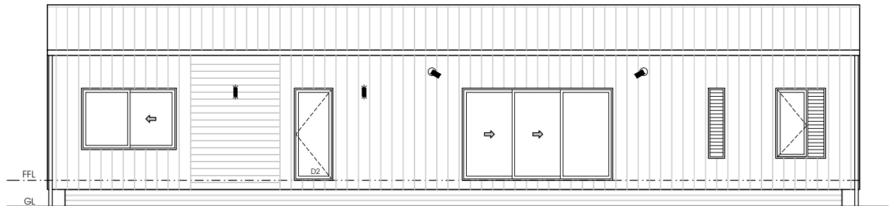
LONG BARN - SPEC HOME 2018 ELEVATION 4
