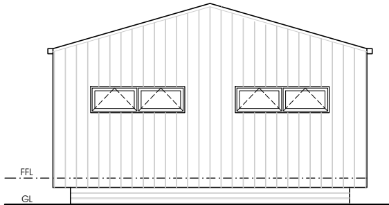
LONG BARN - SPEC HOME 2018 ELEVATION 1
